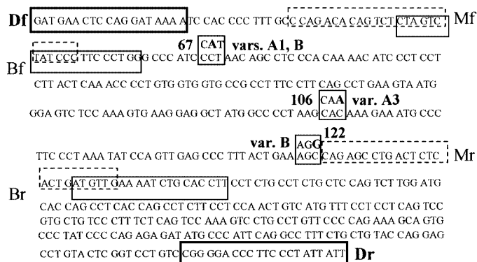
Figure 1. Nucleic acid sequence of Exon VII of the bovine \beta -casein gene, variant A 2 . Target point mutations that differentiate alleles A 1 (codon 67), A 3 (codon 106), and B (codons 67 and 122) are indicated, as well as annealing sequences of the three primer pairs used (see Materials and Methods): Damiani.for (Df) – Damiani.rev (Dr) (thick lines), Medrano.for (Mf) – Medrano.rev (Mr) (dashed lines), and Beta.for (Bf) – Beta.rev (Br) (thin lines). Note that Exon VII is entirely amplified with primer combination Df-Dr.
